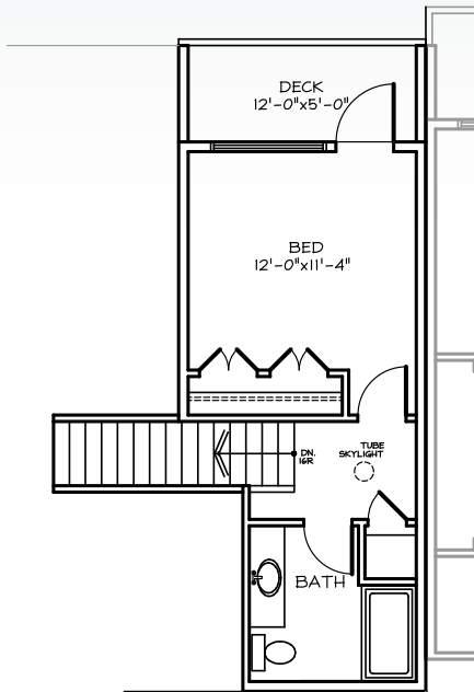
UPPER FLOOR PLAN 310 SQ. FT.
