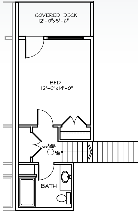
UPPER FLOOR PLAN 322 SQ. FT.
