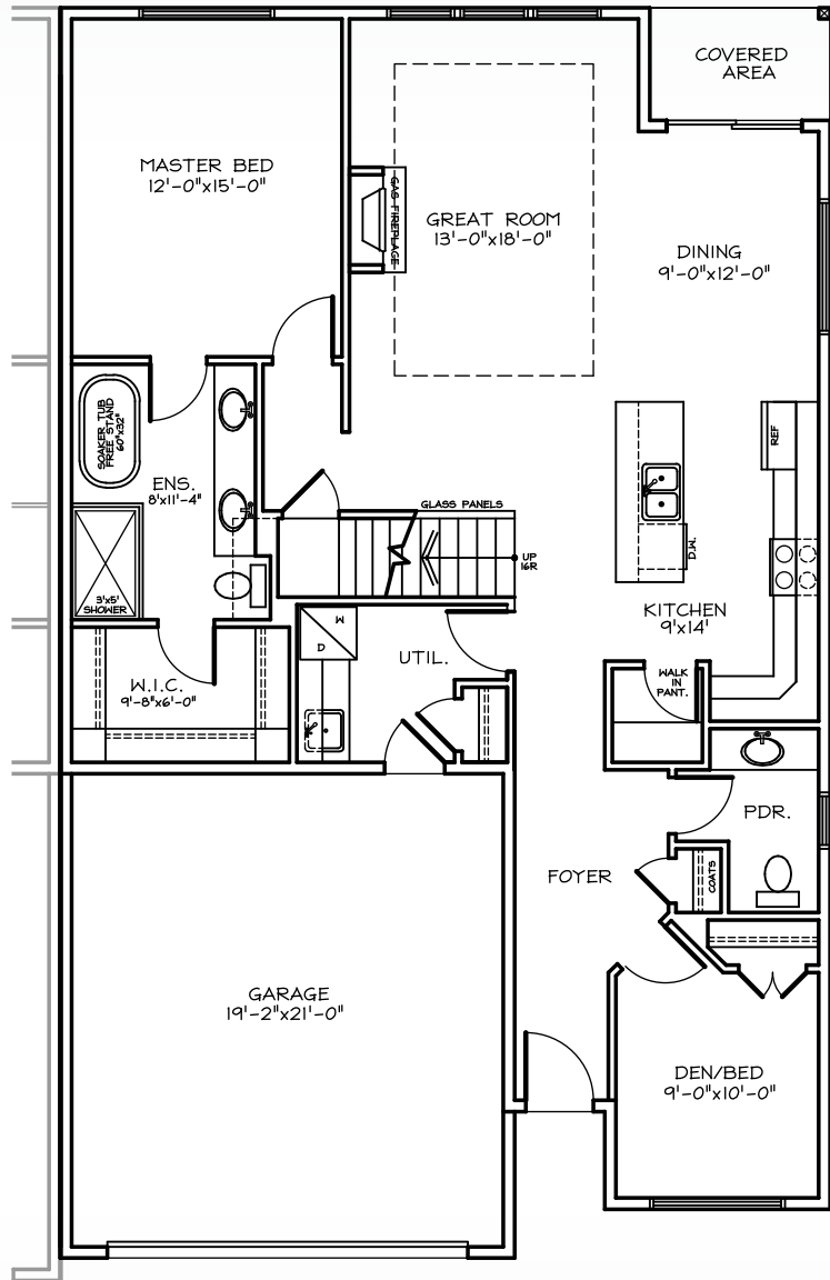
MAIN FLOOR PLAN 1383 SQ. FT. 1705 SQ. FT. TOTAL
