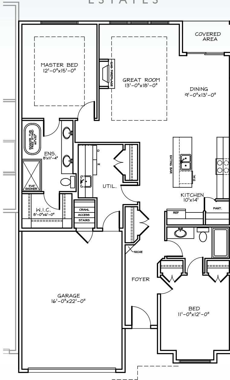
MAIN FLOOR PLAN 1437 SQ. FT.
