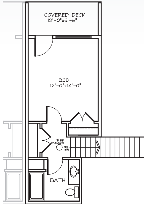
UPPER FLOOR PLAN 322 SQ. FT.
