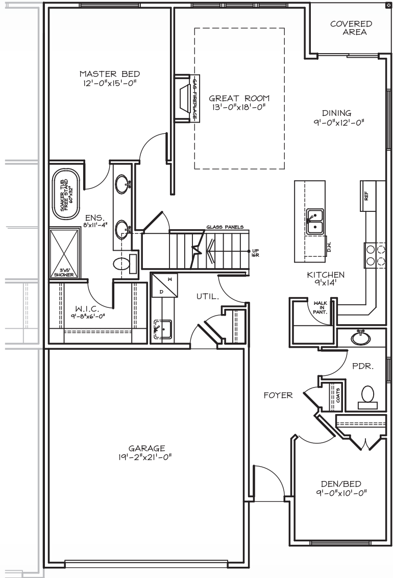
MAIN FLOOR PLAN 1383 SQ. FT. 1705 SQ. FT. TOTAL
