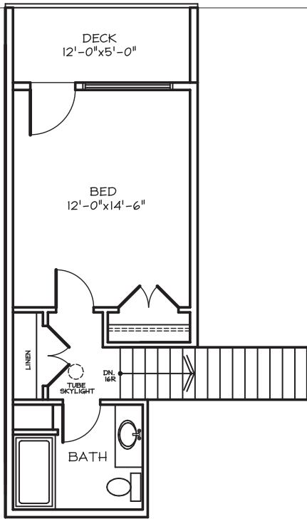
UPPER FLOOR PLAN 322 SQ. FT.
