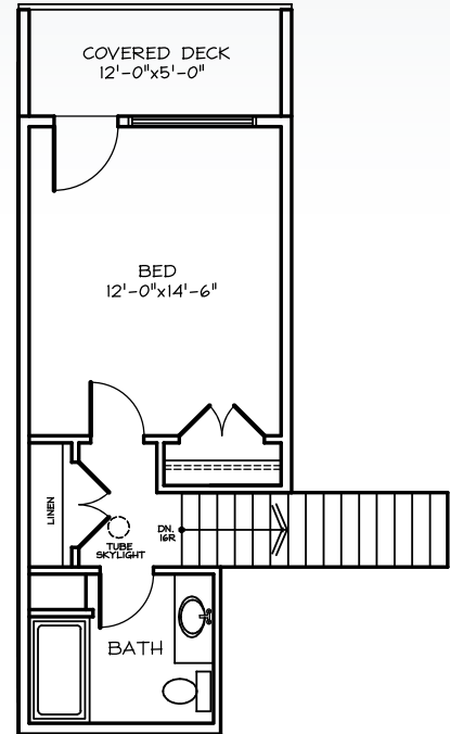
UPPER FLOOR PLAN 322 SQ. FT.
